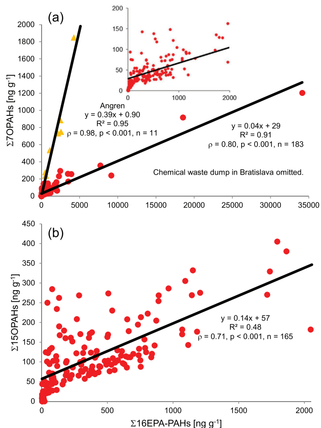
FIGURE 1 Relationship of the concentrations of \Sigma 16\text{EPA-PAHs} with those of (a) the \Sigma 7\text{OPAHs} in 183 topsoils and (b) the \Sigma 15\text{OPAHs} in 165 topsoils from a global data set (the chemical waste dump in Bratislava with a \Sigma 16\text{EPA-PAH} concentration of 230,000 \text{ ng g}^{-1} was omitted). The 11 samples from an industrial area in Angren, Uzbekistan, showed a different relationship of the \Sigma 16\text{EPA-PAH} with the \Sigma 7\text{OPAH} concentrations and are therefore shown separately with triangles. The inset figure magnifies the lower \Sigma 16\text{EPA-PAH} concentration range. The axes of the inset figure have the same legends as those of the main figure. Note the different axis scalings
