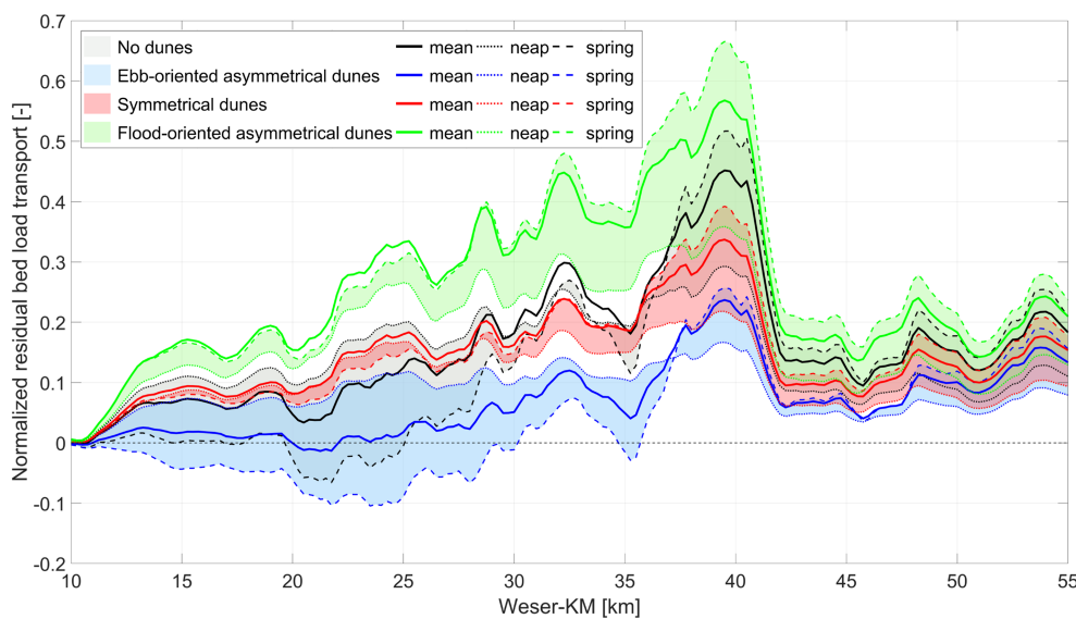
FIGURE 7 This is zoomed in on section III and IV (cf. Figure 6b) to highlight the effect of mean, neap, and spring tidal energy conditions on RBLT for discharge of 450 m 3 /s [Color figure can be viewed at wileyonlinelibrary.com]
