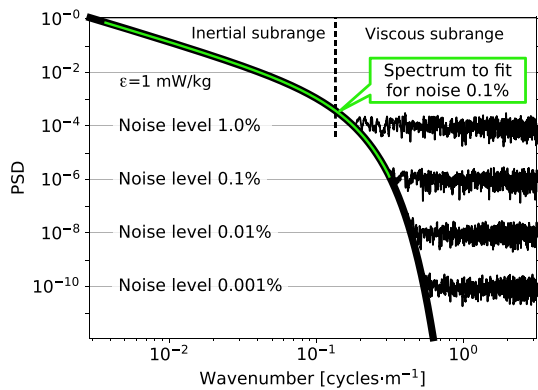
Figure 12. Schematics of power spectra measured with different resolutions. Instrumental noise will cut the measured spectrum as demonstrated by the green line.
