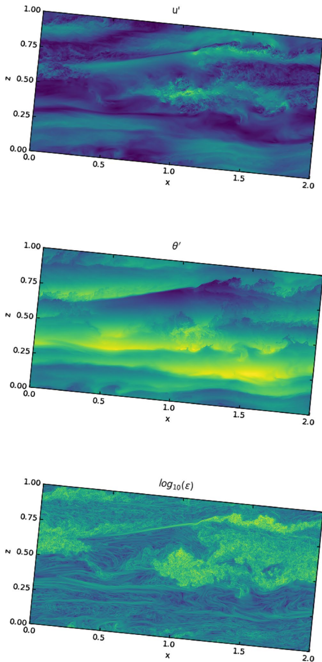
Figure 1. Example of 2D-fields derived by direct numerical simulation (DNS). DNS-Time = 11.5 ( \sim developed turbulence). Lighter colors correspond to higher values.
