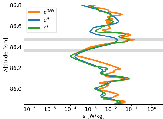
Figure 3. Same as Figure 2 but for smaller altitude range.
