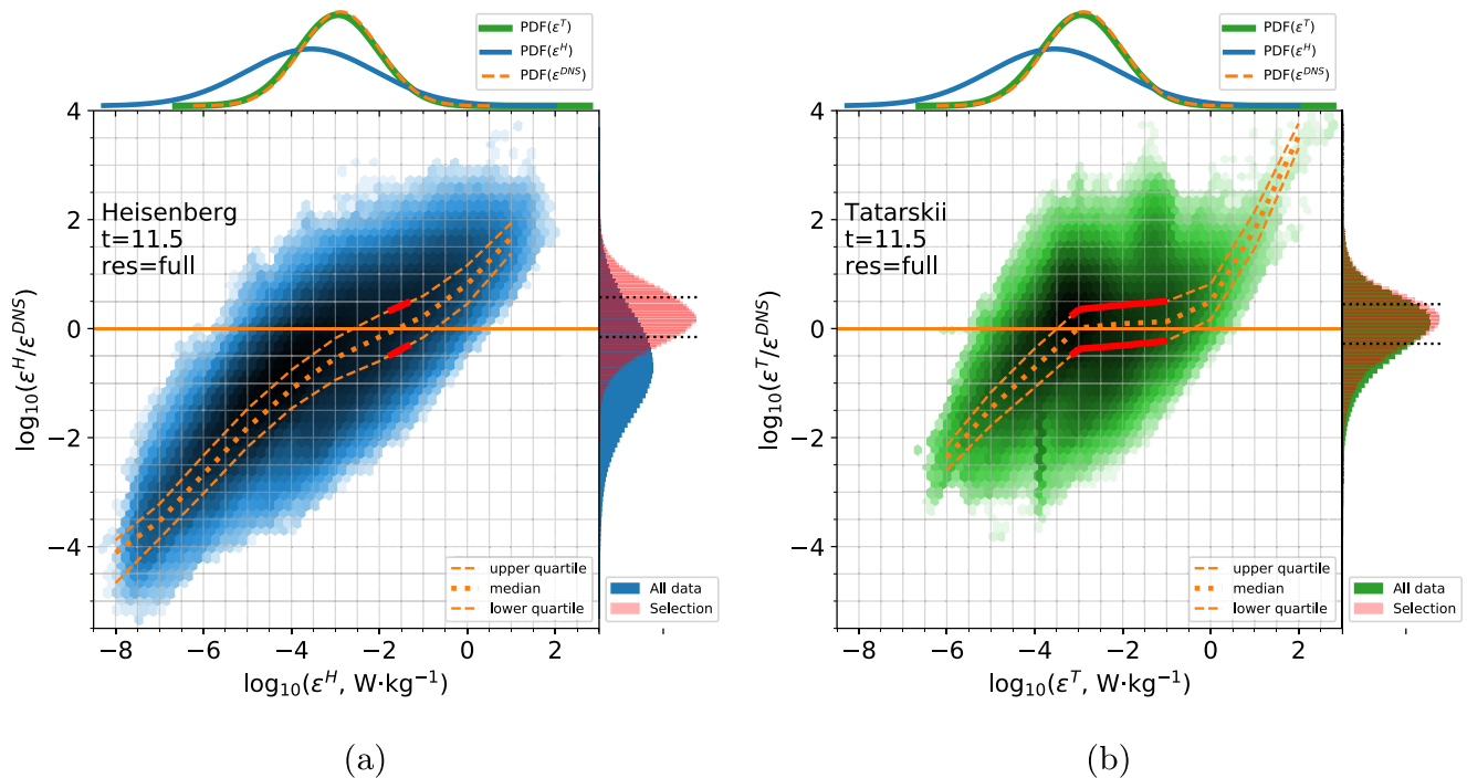
Figure 19. Distributions of the derived energy dissipation rates and of the errors (represented by the ratios \epsilon^{H,T}/\epsilon^{DNS} ) in logarithmic scale. The left (a) and right (b) subfigures are for the Heisenberg and Tatarskii models, respectively. Middle panels: Bi-dimensional histograms of the derived energy dissipation rates ( \epsilon^{H,T} ) and of the measurement errors ( \epsilon^{H,T}/\epsilon^{DNS} ). Solid horizontal lines show the ratio \epsilon^{H,T}/\epsilon^{DNS} = 1 . The dashed lines show upper and lower quartiles of the respective ratio \epsilon^{H,T}/\epsilon^{DNS} , that is, the area between dashed lines shows the interquartile range for the \epsilon -derivation error. The dotted line shows the median error. Upper panels: Distributions of \epsilon^H , \epsilon^T , and \epsilon^{DNS} in blue, green, and orange, respectively. Right-hand-side panels: Distributions of the ratios \epsilon^{H,T}/\epsilon^{DNS} . Red color in the mid- and right-panels shows selection of data with errors within one decade around the zero-line: -0.5 < \log_{10}(\epsilon^{H,T}/\epsilon^{DNS}) < 0.5 . Red histograms show distributions of errors for the selection of data. The black dotted lines show the lower and upper quartiles for red histograms.
