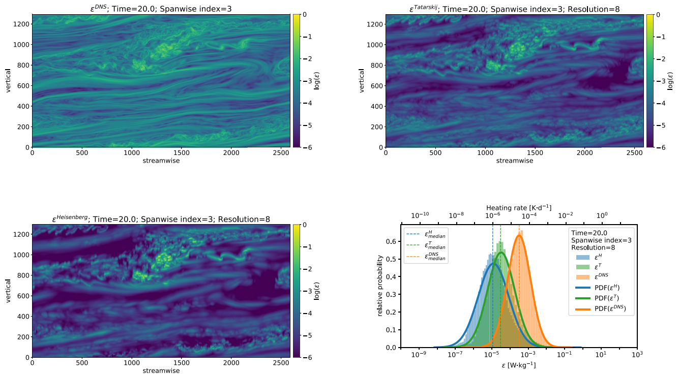
Figure 16. Same as Figure 11, but for noised spectra with 4.5 decades of visible power within the viscous subrange (noise level of 0.01%).
