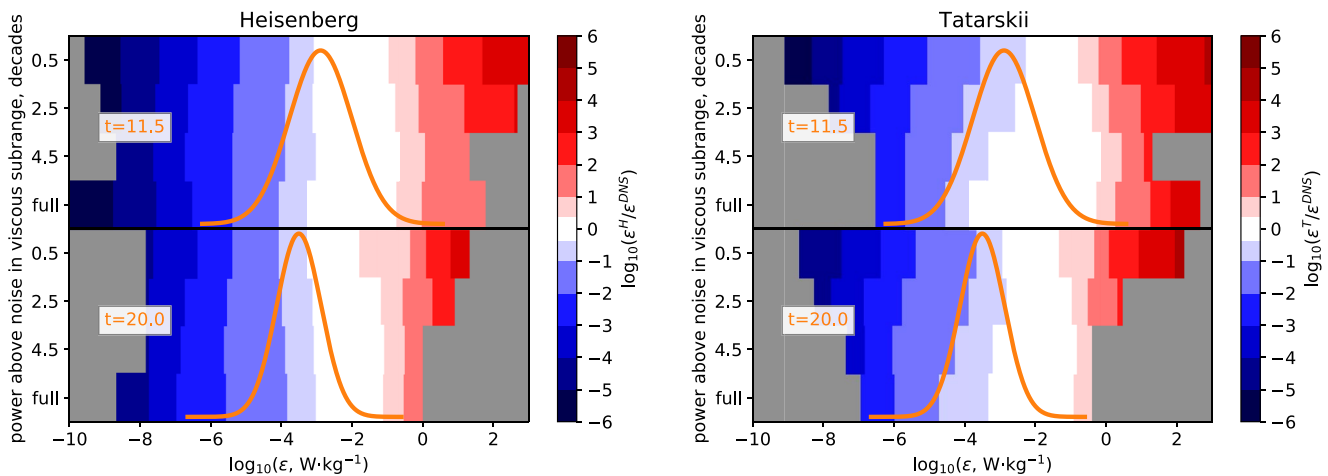
Figure 21. Ratios of the derived to true energy dissipation rates in logarithmic scale: \log_{10}(\epsilon^{\text{H},T}/\epsilon^{\text{DNS}}) shown by colors as a function of \epsilon^{\text{H},T} -value (abscissa) and spectral resolution (ordinate). White color shows range of \epsilon^{\text{H},T} -values where their error falls within half-decade interval: -0.5 < \log_{10}(\epsilon^{\text{H},T}/\epsilon^{\text{DNS}}) < 0.5 . Red and blue colors show regions where derived \epsilon^{\text{H},T} are over- and underestimated, respectively. Orange Gaussians schematically show \text{PDF}(\epsilon^{\text{DNS}}) .
