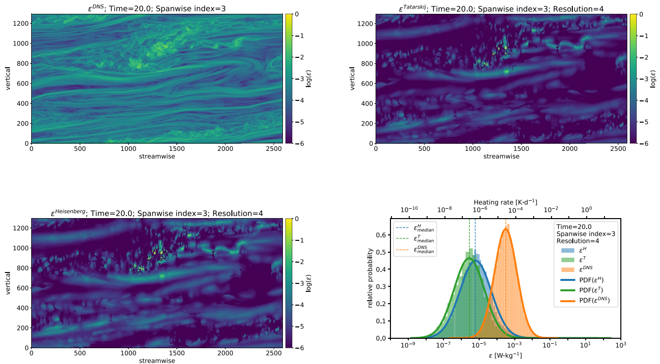
Figure 18. Same as Figure 11, but for noised spectra with 0.5 decades of visible power within the viscous subrange (noise level of 1%).
