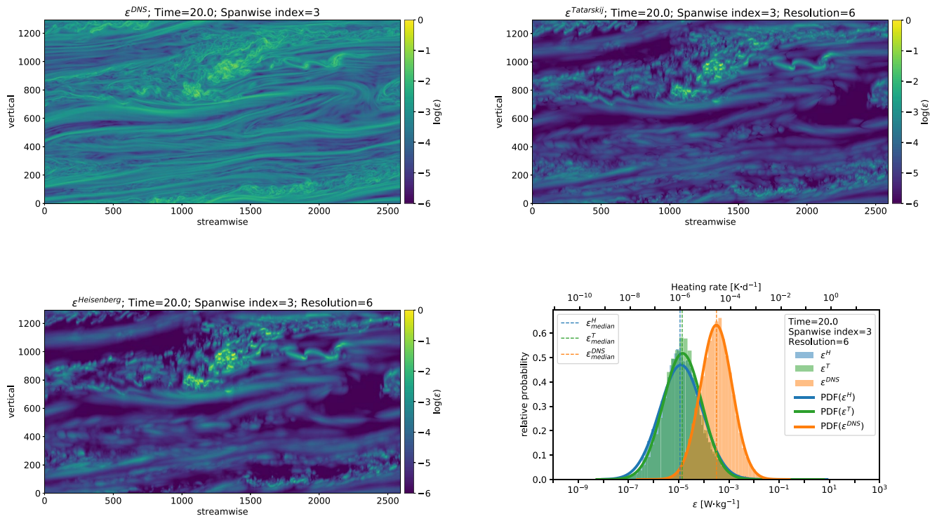
Figure 17. Same as Figure 11, but for noised spectra with 2.5 decades of visible power within the viscous subrange (noise level of 0.1%).
