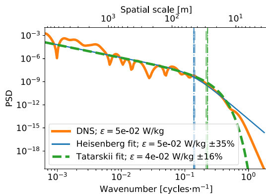
Figure 5. Example of power spectra which yield the \varepsilon -profiles shown in Figure 2 taken at an altitude of 85.413 km. Orange, blue, and green lines show the direct numerical simulation (DNS), Heisenberg, and Tatarskii data. Bold vertical dashed lines show the inner scales ( l_0 = 2\pi/k_0 ) derived from the fit of the Heisenberg ( l_0^H = 9.9(v^3/\varepsilon^H)^{1/4} ) and Tatarskii ( l_0^T = 7.06(v^3/\varepsilon^T)^{1/4} ) models in blue and green, respectively. Vertical dashed-dotted lines show the inner scales derived from the DNS data ( \varepsilon^{\text{DNS}} -value) based on the Heisenberg model ( l_0^H = 9.9(v^3/\varepsilon^{\text{DNS}})^{1/4} ) and Tatarskii ( l_0^T = 7.06(v^3/\varepsilon^{\text{DNS}})^{1/4} ) model in blue and green, respectively.
