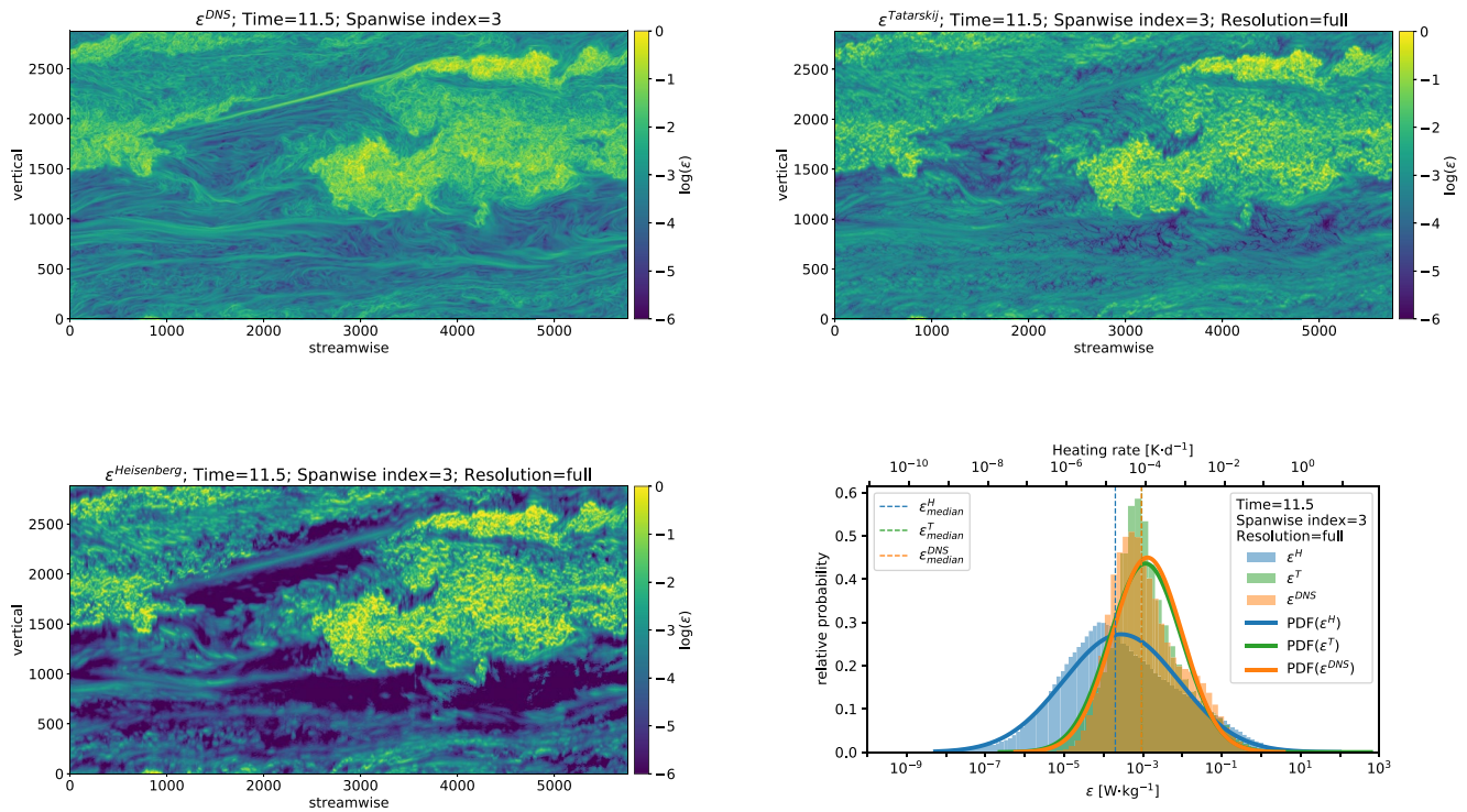
Figure 10. 2D-fields of the kinetic energy dissipation rates. Panel (a) shows the “true” direct numerical simulation (DNS) data used as reference (the same as Figure 1c). DNS-time = 11.5, that is, for well-developed turbulence. Panels (b) and (c) show analysis results using Tatarskij and Heisenberg models, respectively. Lighter colors correspond to higher \epsilon -values. Panel (d) shows the same data as in panels (a–c), but as histograms of \epsilon -distributions and fitted PDFs. Vertical dashed lines show medians of corresponding data sets (here the DNS and Tatarskij results almost coincide and are hardly distinguishable).
