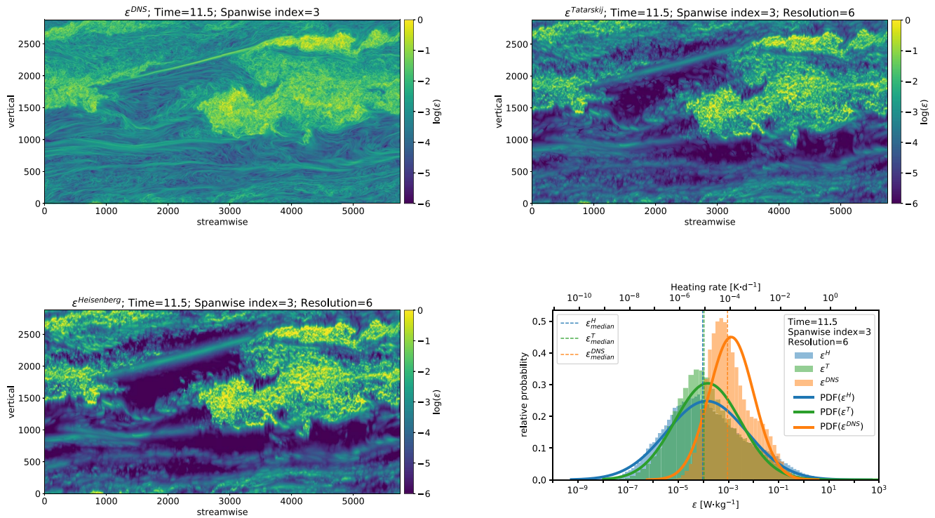
Figure 14. Same as Figure 10, but for noised spectra with 2.5 decades of visible power within the viscous subrange (noise level of 0.1%).
