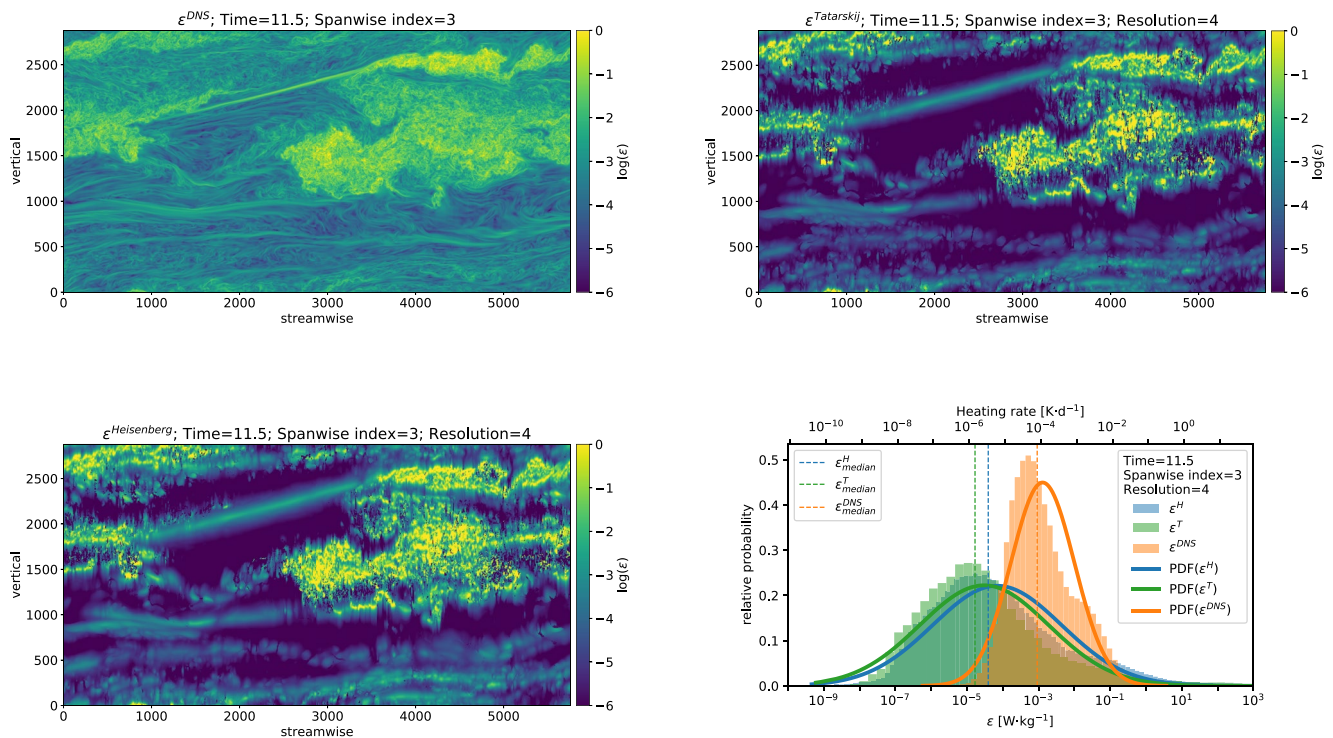
Figure 15. Same as Figure 10, but for noised spectra with 0.5 decades of visible power within the viscous subrange (noise level of 1%).
