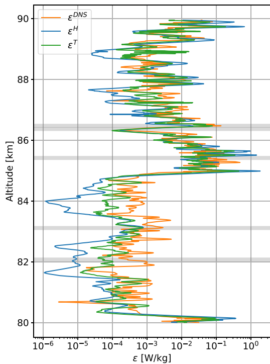
Figure 2. Example of vertical profiles of the derived energy dissipation rates. The orange profile shows the direct numerical simulation data, whereas the blue and green profiles show the analysis results using the Heisenberg and Tatarskii spectral models, respectively. Gray bold horizontal lines mark altitudes where power spectra are taken from for demonstration in Section 5.2.
