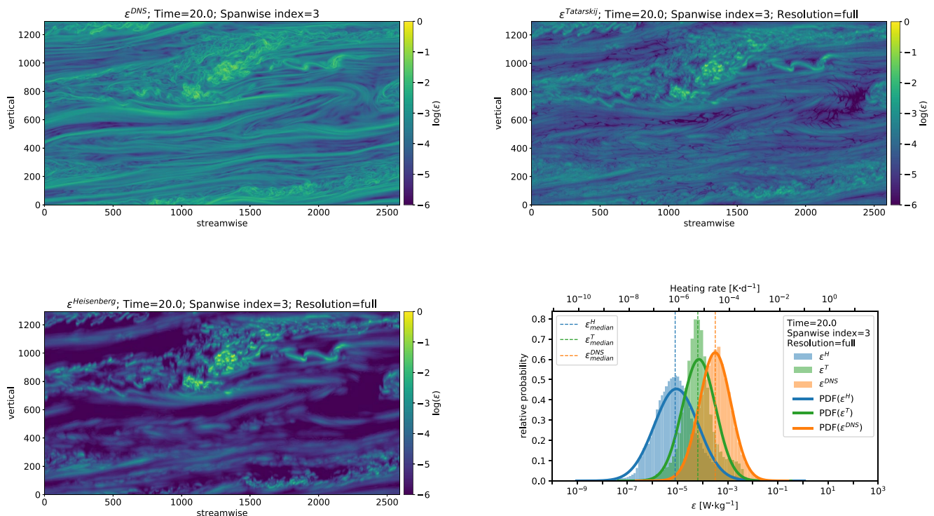
Figure 11. Same as Figure 10, but for direct numerical simulation -time = 20.0, that is, for decaying turbulence.
