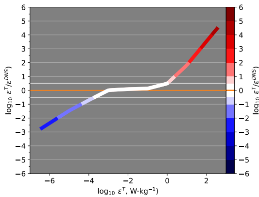
Figure 20. Example of the derived \epsilon -error represented by the ratio in logarithmic scale: \log_{10}(\epsilon^T/\epsilon^{\text{DNS}}) . Color-coding of both line and colorbar mirrors the ordinate axis. White color shows range of \epsilon^{\text{H},T} -values where their error falls within half-decade interval: -0.5 < \log_{10}(\epsilon^{\text{H},T}/\epsilon^{\text{DNS}}) < 0.5 . Red and blue colors show regions where derived \epsilon^{\text{H},T} are over- and underestimated, respectively.
