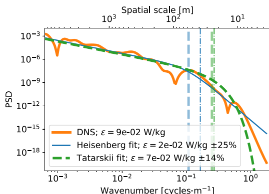
Figure 7. Same as Figure 5, but for an altitude of 86.470 km.
