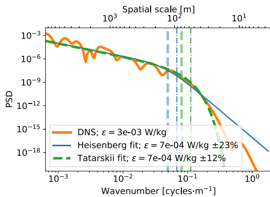
Figure 8. Same as Figure 5, but for an altitude of 83.109 km.
