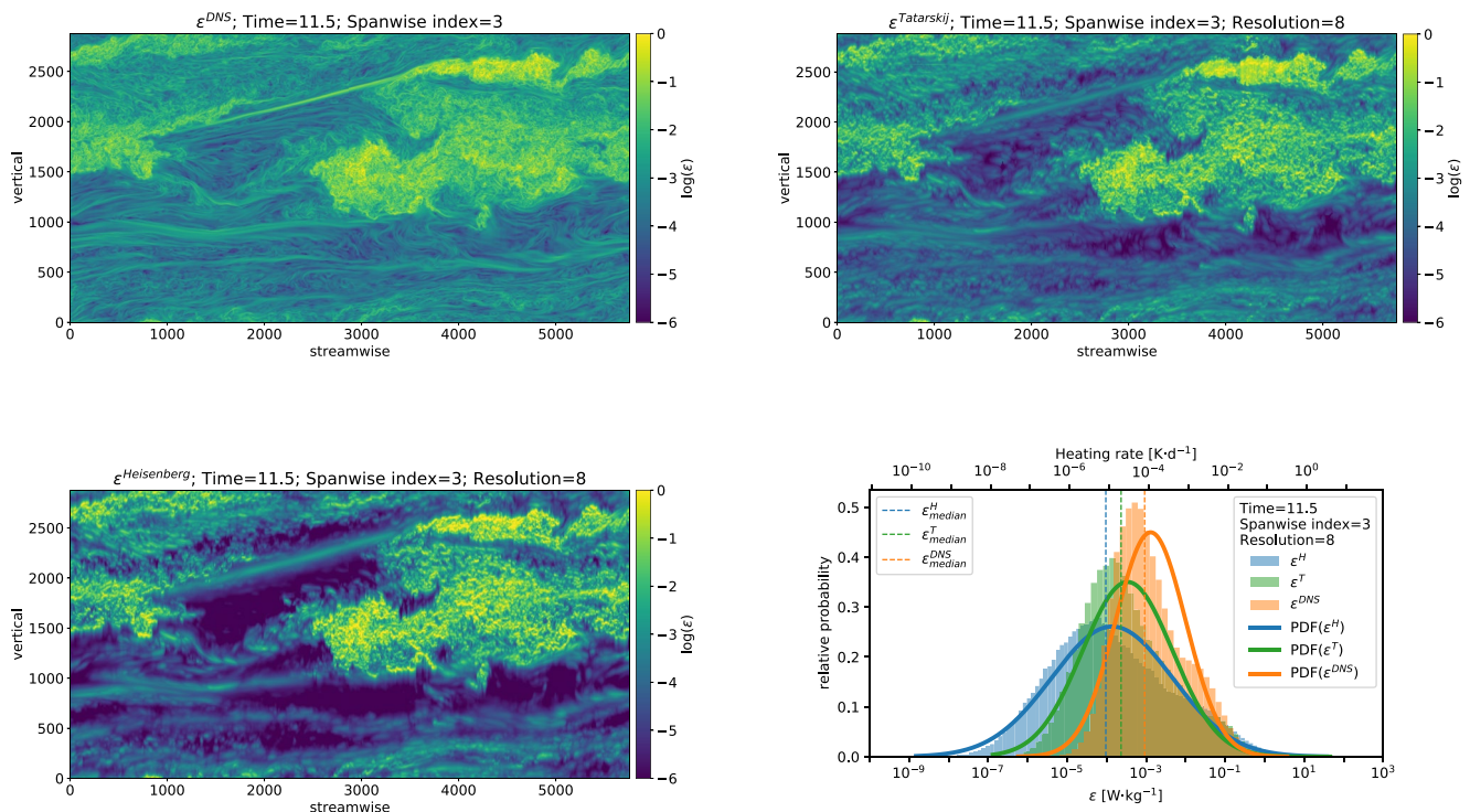
Figure 13. Same as Figure 10, but for noised spectra with 4.5 decades of visible power within the viscous subrange (noise level of 0.01%).
