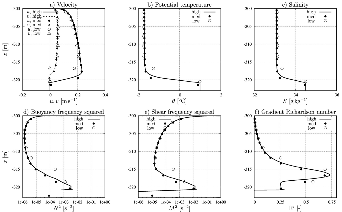
Figure 9. Vertical profiles of (a) velocity, (b) potential temperature, (c) salinity, (d) buoyancy frequency squared, (e) shear frequency squared and (f) gradient Richardson number after 14 days of simulation using the default scenario with high resolution of k_{\max} = 500 layers (lines), a medium resolution of k_{\max} = 50 layers (black symbols) and a low resolution of k_{\max} = 25 layers (open symbols).
