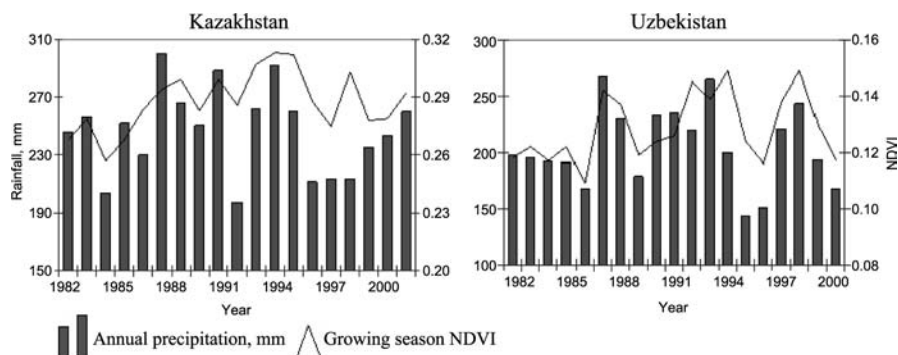
Figure 2. Time-series of annual precipitation and the mean growing season NDVI for Kazakhstan and Uzbekistan
