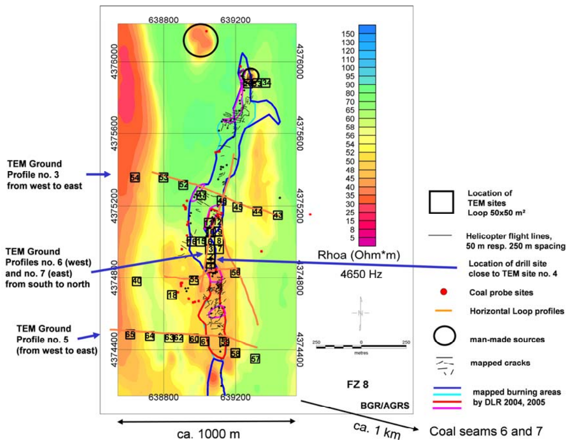
Figure 3: Map of apparent resistivity R_{\rho a} ( \text{Ohm}\cdot\text{m} ) at a frequency of 4,650 Hz, derived from airborne survey over FZ 8. The locations of TEM sites crossing the active parts of the FZ are marked by black squares, including a drilling site close to TEM site no. 4 (see Chapter 3.2).
