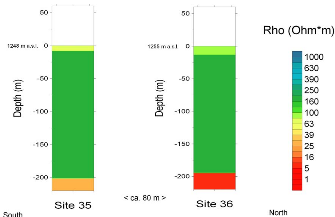
Figure 8: One-dimensional inversion models derived from TEM data outside FZ 8's burning zones over unaffected coal seams nos. 6 and 7 about 1 km southeast of FZ 8
