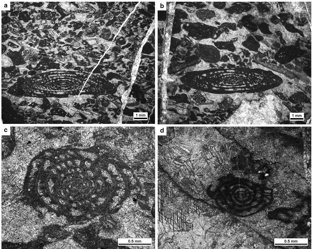
Fig. 4 Photomicrographs of fusuline foraminifera of the studied limestone samples. a,b Pseudofusulina sp. (inv.-no. GEOCU 2020 KW-01). c,d Misellina (M.) termieri (inv.-no. GEOCU 2020 KW-02)
