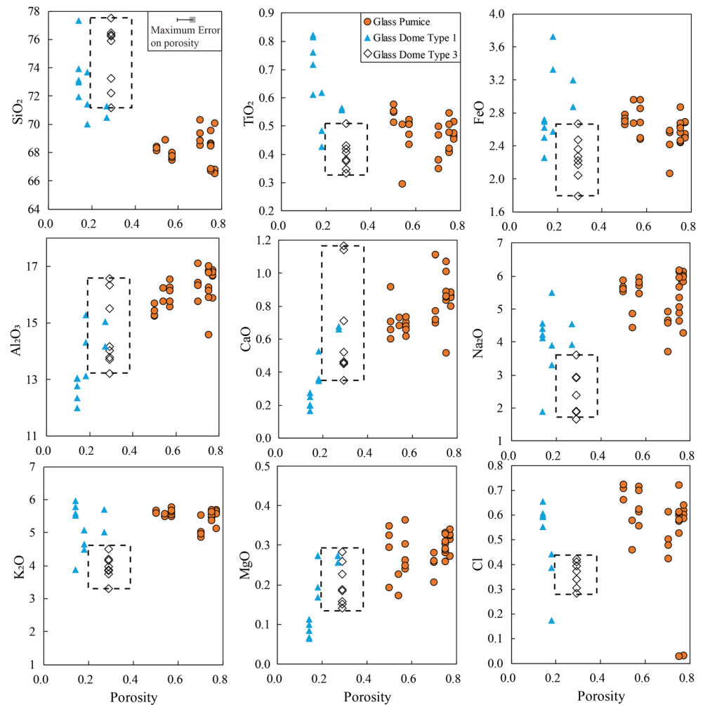
Fig. 8 Evolution of interstitial glass composition with whole pyroclast porosity. Orange circles: pumice glass. The dashed boxes show the range of porosities observed in the heterogeneous Type 3 dome pyroclasts
