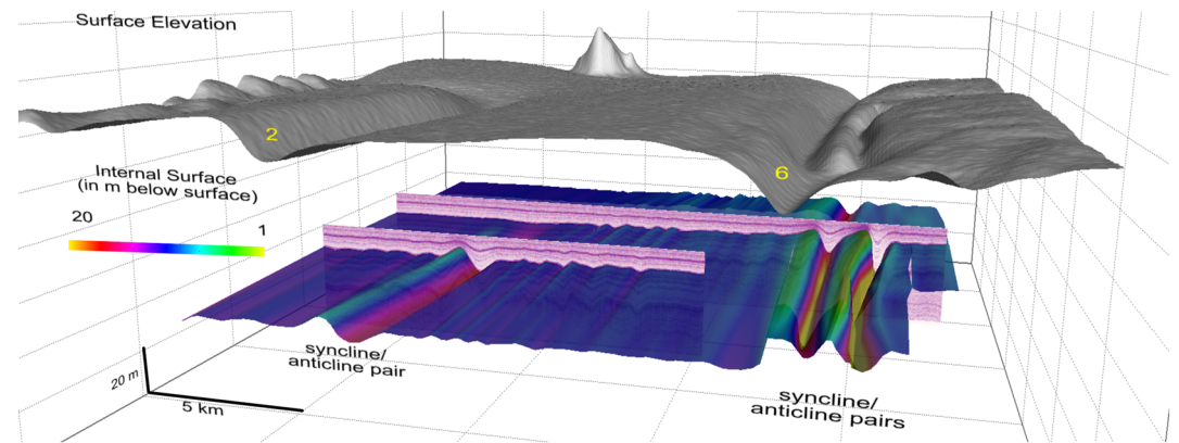
Figure 7. Perspective view into the along-flow direction. Surface depressions of Ice Shelf Channels 2 and 6 are shown in gray. An internal reflection surface interpolated from all radar cross sections is shown in color as depth below surface. The two surfaces are vertically offset to improve visibility. Syncline/anticline pairs associated with the surface depressions are the dominant patterns in the shallow stratigraphy of all cross sections.
