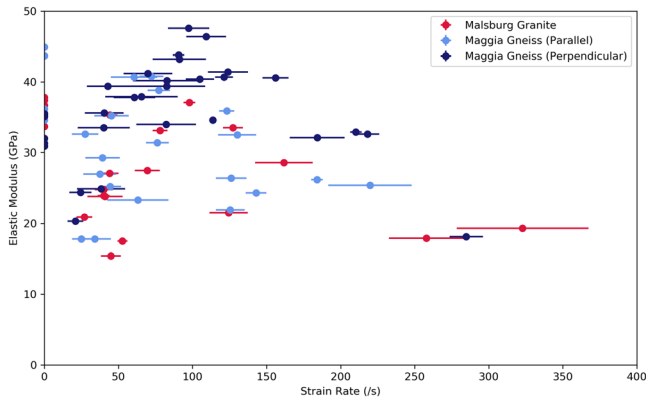
Figure 3. Elastic modulus from quasi-static and dynamic testing at various strain rates. Data presented with a logarithmic x axis are shown in supporting information Figure S3.
