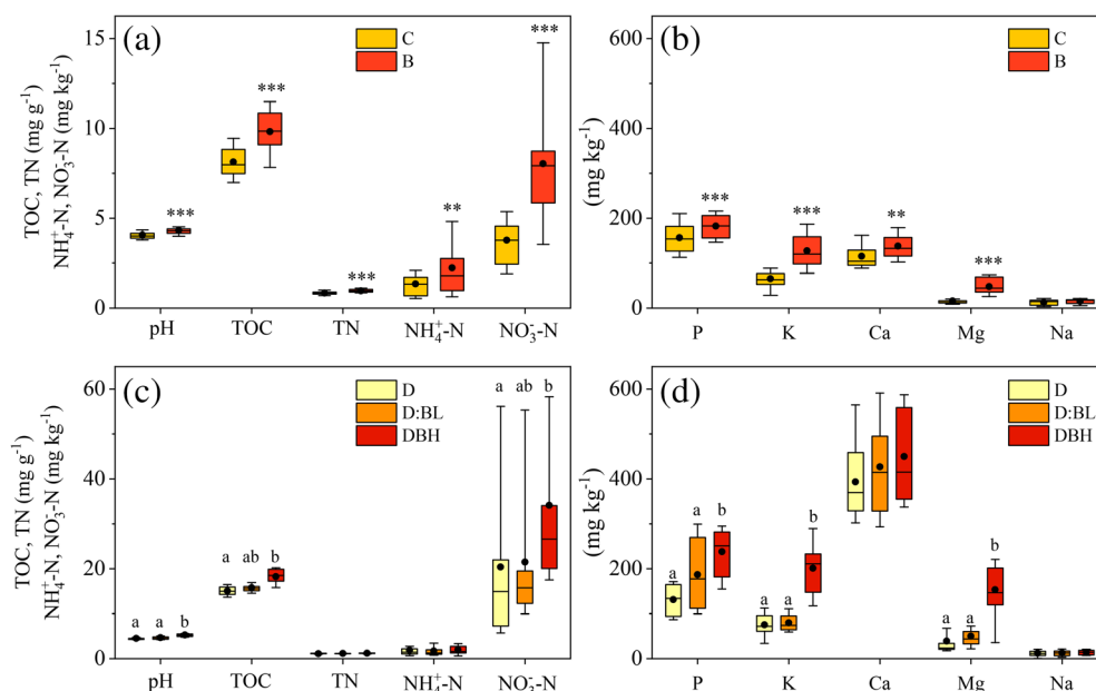
FIGURE 1 pH, total organic carbon (TOC), total nitrogen (TN), ammonium ( \text{NH}_4^+\text{-N} ) and nitrate ( \text{NO}_3^-\text{-N} ) concentrations (a, c) and plant available nutrient concentrations (b, d) in the surface soils of the different treatments at the fallow (a, b) and the cornfield (c, d) sites. Presented are data from all sampling times during the field experiment lasting from winter 2012/2013 to summer 2014. Boxes represent the 25th to 75th percentiles and whiskers are the 10th to 90th percentiles. The horizontal line in each box represents the median value; the closed circle associated with each box represents the mean value ( n = 24\text{--}45 ). The asterisks indicate a significant ( t -test, ** = p < 0.01 , *** = p < 0.001 ) difference between the control (C) and the biochar treatments (B). The different lowercase letters indicate significantly different subgroups (ANOVA, Tukey honestly significant difference [HSD] post-hoc, p < 0.05 ) [Color figure can be viewed at wileyonlinelibrary.com ]
