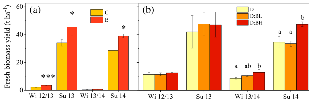
FIGURE 2 Yield of fresh aboveground plant biomass during the four cropping seasons of the field experiment at the fallow (a) and the cornfield (b) sites. During the winter seasons of 2012/2013 and 2013/2014 the fields were cropped with winter wheat and winter rye, respectively. Corn was grown during the two summer seasons in 2013 and 2014. Given are mean values ( n = 3 ) with one standard deviation. The asterisks indicate a significant ( t -test, * = p < 0.05 , *** = p < 0.001 ) difference between the control (C) and the biochar (B) treatments at the fallow site. The different lowercase letters indicate significantly different subgroups (ANOVA, Tukey honestly significant difference [HSD] post-hoc, p < 0.05 ) at the cornfield site. BH, biochar high; BL, biochar low; D, digestate [Color figure can be viewed at wileyonlinelibrary.com]
