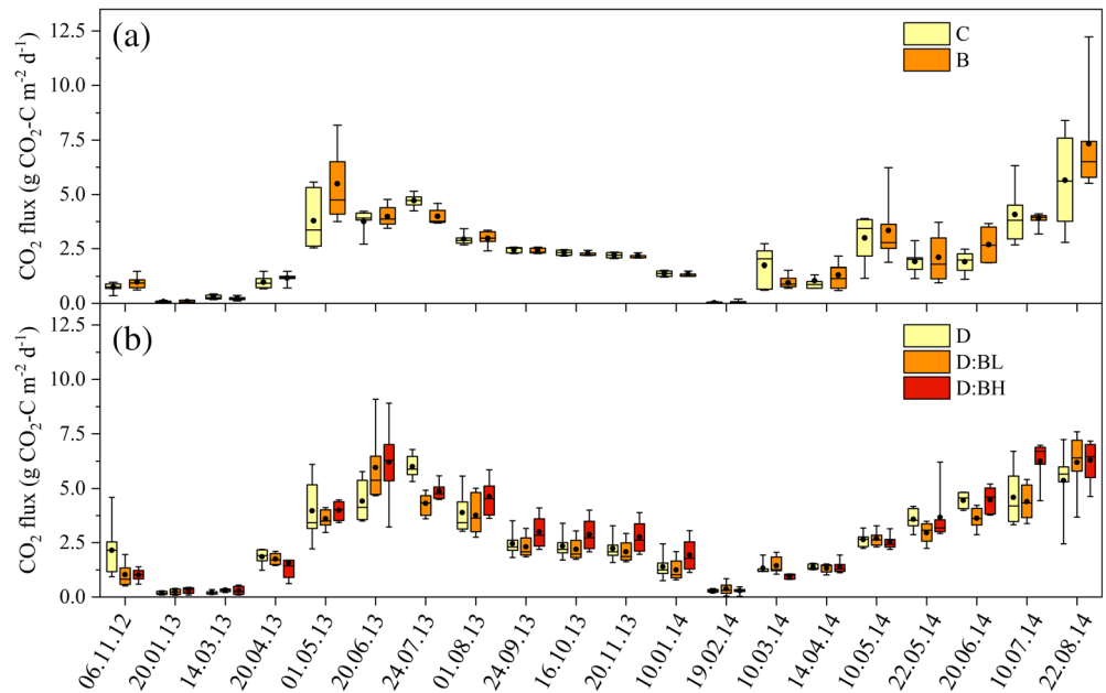
FIGURE 4 Carbon dioxide fluxes between November 2012 and August 2014 from the different treatments at the fallow (a) and the cornfield (b) sites. The boxes represent the 25th to 75th percentiles and whiskers the 10th to 90th percentiles. The horizontal line in each box represents the median value; the closed circle associated with each box represents the mean value. B, biochar; BH, biochar high; BL, biochar low; C, control; D, digestate [Color figure can be viewed at wileyonlinelibrary.com ]
