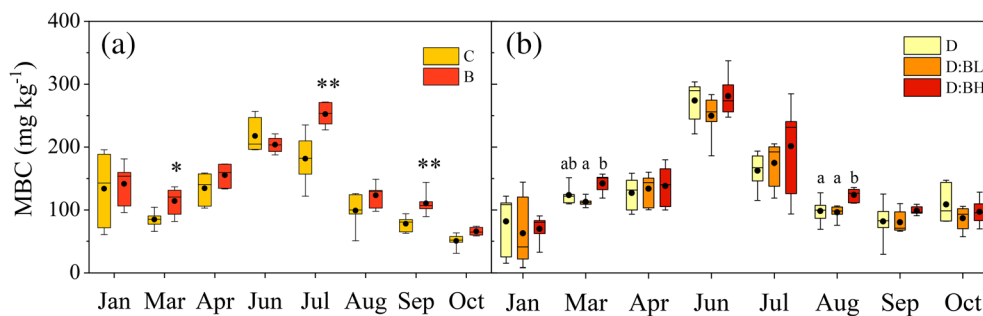
FIGURE 3 Soil microbial biomass carbon (MBC) in surface soils of the fallow (a) and the cornfield (b) plots between January and October 2013. The boxes represent the 25th to 75th percentiles and whiskers the 10th to 90th percentiles. The horizontal line in each box represents the median value; the closed circle associated with each box represents the mean value. The asterisks in (a) indicate a significant ( t -test, * = p < 0.05 , ** = p < 0.01 ) difference between the C and B treatments. The different lowercase letters in (b) indicate significantly different subgroups (ANOVA, Tukey honest significant difference [HSD] post-hoc, p < 0.05 ). BH, biochar high; BL, biochar low; D, digestate [Color figure can be viewed at wileyonlinelibrary.com]
