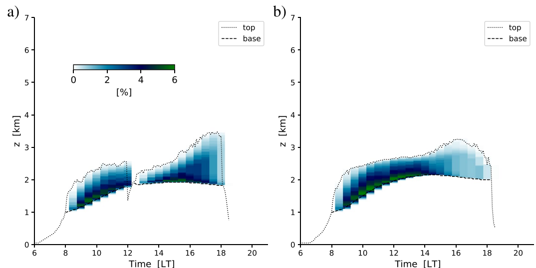
Figure 17. Time height plot of EDMF cloud fraction (a) experiment B m and (b) experiment B θ v for 11 June 2016. The Lifting Condensation Level (black dashed) and maximum plume termination height (black dotted) are also shown, for reference.
