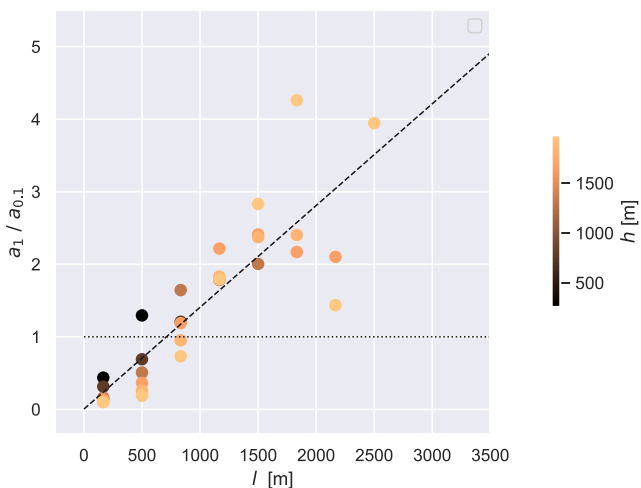
Figure 5. Ratio of cluster area at mixed layer top versus that at surface layer top, as a function of cluster size l , as sampled in a LASSO LES of shallow cumulus observed on 11 June 2016 at the Atmospheric Radiation Measurement Southern Great Plains site. The data points represent averages over 2 hours at a bin-width of 333 m, with the color indicating mixed layer depth h . The Pearson correlation coefficient is 0.86. The black dashed line indicates the least squares linear fit.
