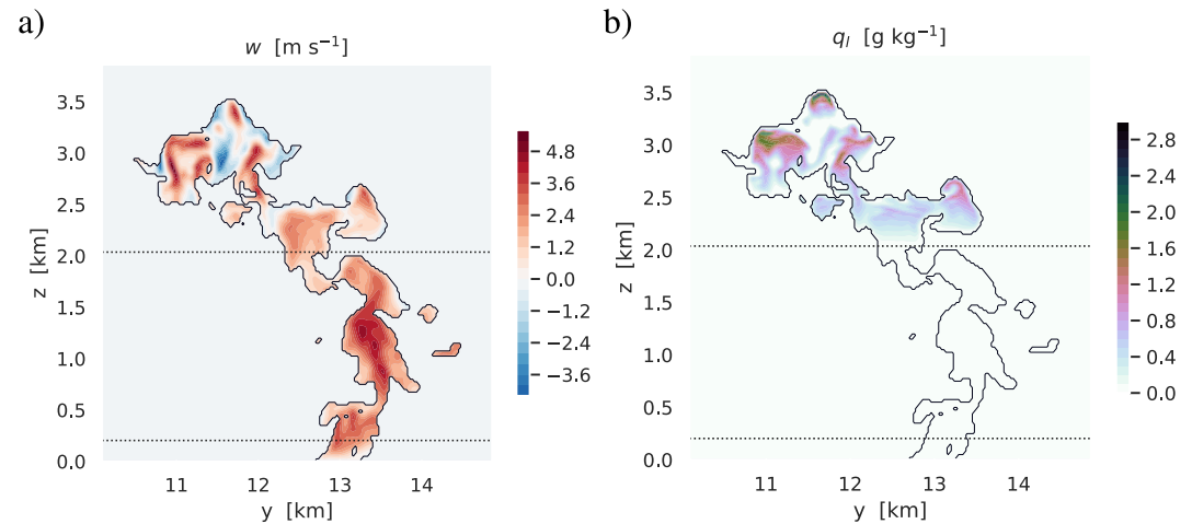
Figure 1. Vertical cross section through a surface-rooted convective plume as sampled from a LASSO LES of shallow cumulus observed on 11 June 2016 at the Atmospheric Radiation Measurement Southern Great Plains site. The simulation and cluster sampling are fully described by Griewank et al. (2021), as briefly summarized in Sections 3 and 4. Shown are (a) object vertical velocity w and (b) cloud liquid water q_l . The cluster outline is indicated by the solid black line. The two dotted lines indicate mixed-layer top ( z/h = 1 ) and surface layer top ( z/h = 0.1 ). The local maxima in w can be interpreted as thermal cores, forming a chain that makes up the plume.
