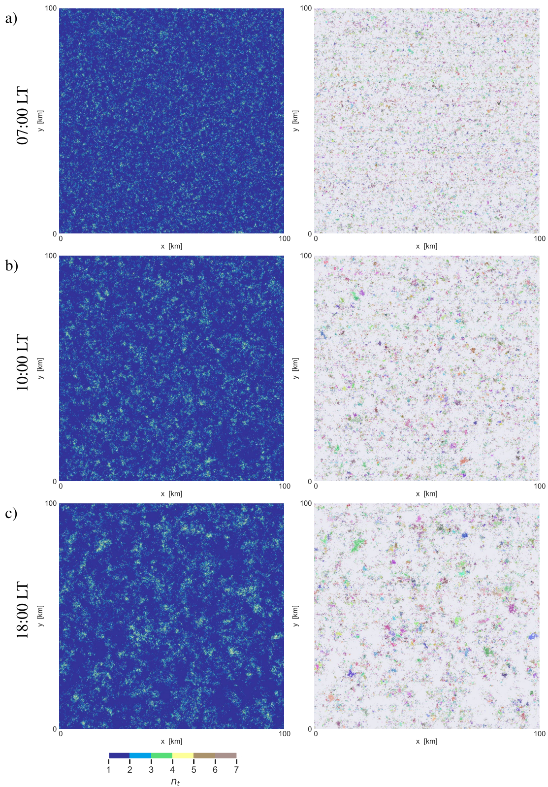
Figure 10. Snapshots of thermal clustering on the BiOMi microgrid at (a) 07:00 local time (LT), (b) 10:00 LT and 18:00 LT during the B experiment for 11 June 2016. These time points correspond to 1, 4, and 12 hr after initialization. Left column: Rasterplot of the total number of thermals per cell, n_t . Right column: The associated cluster mask, with each individual cluster given a unique color. Note that the thermal clusters represent both dry and condensed thermal plumes.
