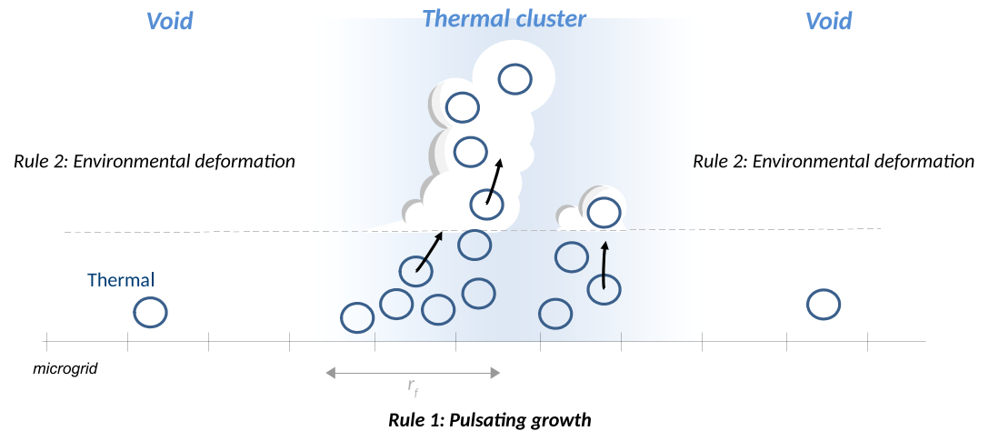
Figure 3. Schematic illustration of the role of Binomials On Microgrids (BiOMi) Rules 1 and 2 in creating long-lived thermal clusters on the microgrid. The impact radius r_f of Rule 1 is indicated for the central microgrid cell, with the associated magnitude f_p indicated by the blue background shading.
