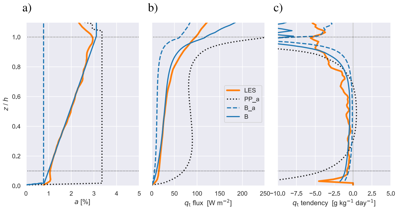
Figure 15. Profiles of average properties of the Super-Scale-break Size Segment ( S^4 ), representing all plumes larger than the scale-break size. (a) Area fraction a , (b) convective q_t flux, and (c) the associated q_t tendencies calculated as the vertical flux convergence. Sampling time is 16:00 local time on 11 June 2016. LES is shown in orange, experiment PP_a in black, and B_a and B in dashed and solid blue, respectively. Height z is normalized by mixed layer depth ( h ).
