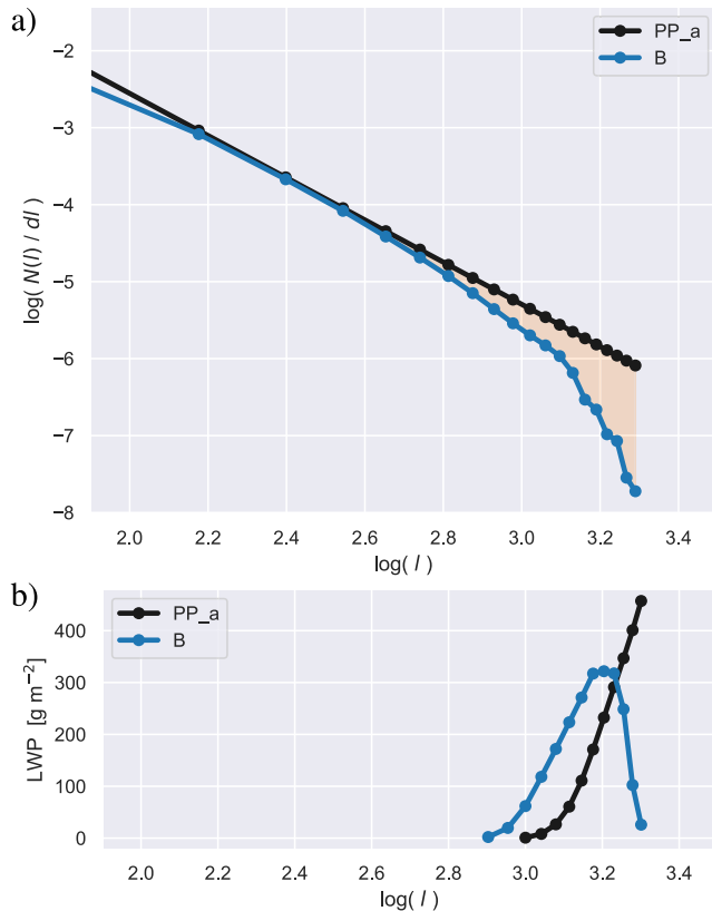
Figure 13. Size densities of (a) plume number N(l) and (b) plume liquid water path for experiments B (blue) and PP_a (black) as time averaged over the period 10:00–12:00 local time on 11 June 2016. The difference in plume number at sizes above the scale break is shaded orange. This size range is referred to as the Super-Scale-break Size Segment ( S^4 ).
