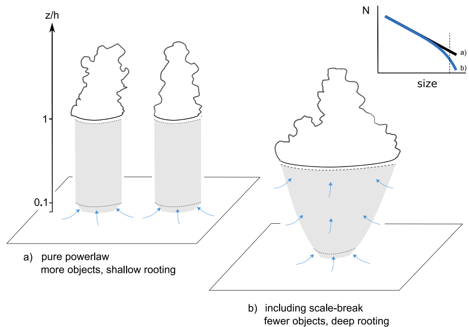
Figure 18. Schematic illustration of the two configurations of plume rooting as applied in the ED(MF) n experiments in this study. (a) Shallow rooting with a pure powerlaw distribution of plume number. (b) Mixed-layer deep rooting for distributions including a scale break. Plume volume within the mixed layer is indicated by the gray shading. Height z is normalized by mixed-layer depth ( h ). Blue arrows indicate dynamic entrainment of mass into the plume. The associated two functional forms of the size distribution of plume number are shown in the inset. The deep rooting configuration (b) is supported by LES results.
