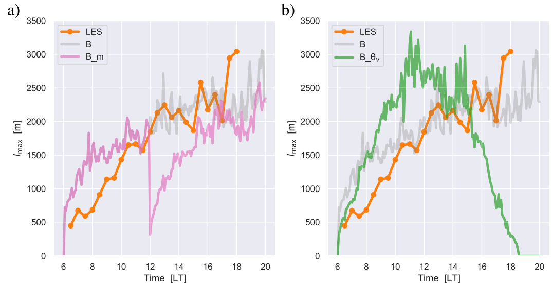
Figure 16. Time series of the largest cluster size l_{\max} for (a) experiment B m (pink) and (b) experiment B θ v (green). Experiment B and LES are also shown, for reference.
