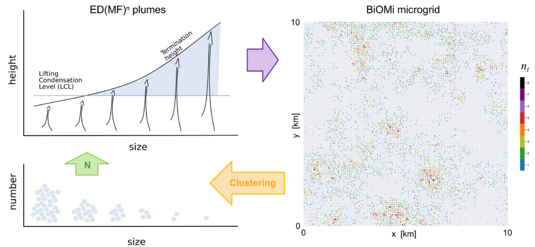
Figure 2. Schematic illustration of the coupling of Binomials On Microgrids (BiOMi) (right) and ED(MF)^n (top left) through an online clustering algorithm (bottom left). The colored arrows indicate the information flow between components, as explained in the text. n_t represents the total number of thermals in a BiOMi microgrid cell (colored).
