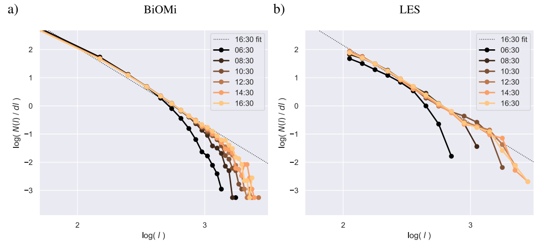
Figure 11. Log-log plot of size densities of cluster number N(l) at 2-hr intervals during 11 June 2016, with size l shown in m. (a) Clusters on the Binomials On Microgrids (BiOMi) microgrid during experiment B. (b) Coherent objects in LASSO LES. Lines represent hourly means around the indicated time-point (local time) for a 100 \times 100 \text{ km}^2 domain. The dotted black line indicates the linear fit f(l) = al + b in log-log space for the size densities at 16:30 local time, as applied to the scaling range 100 < l < 1,000 \text{ m} . The corresponding powerlaw exponents are a = -2.74 for BiOMi and a = -2.77 for LES.
