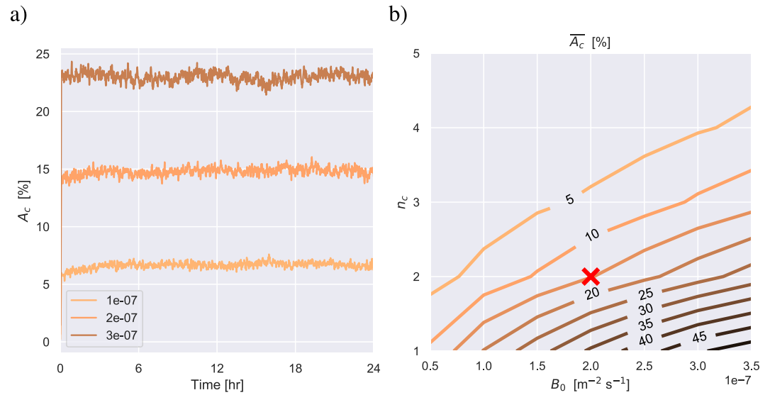
Figure 4. Results from offline experiments with Binomials On Microgrids (BiOMi) on a 100 \times 100 grid. (a) Time series of total cluster area fraction A_c for n_c = 2 and for three experiments with a different B value. (b) Phase-space diagram of time averaged \overline{A_c} (contoured) as a function of thermal birth rate \hat{B} and clustering threshold n_c . The thermal life time \tau is always 300 s. The red marker in (b) indicates the values selected in this study.
