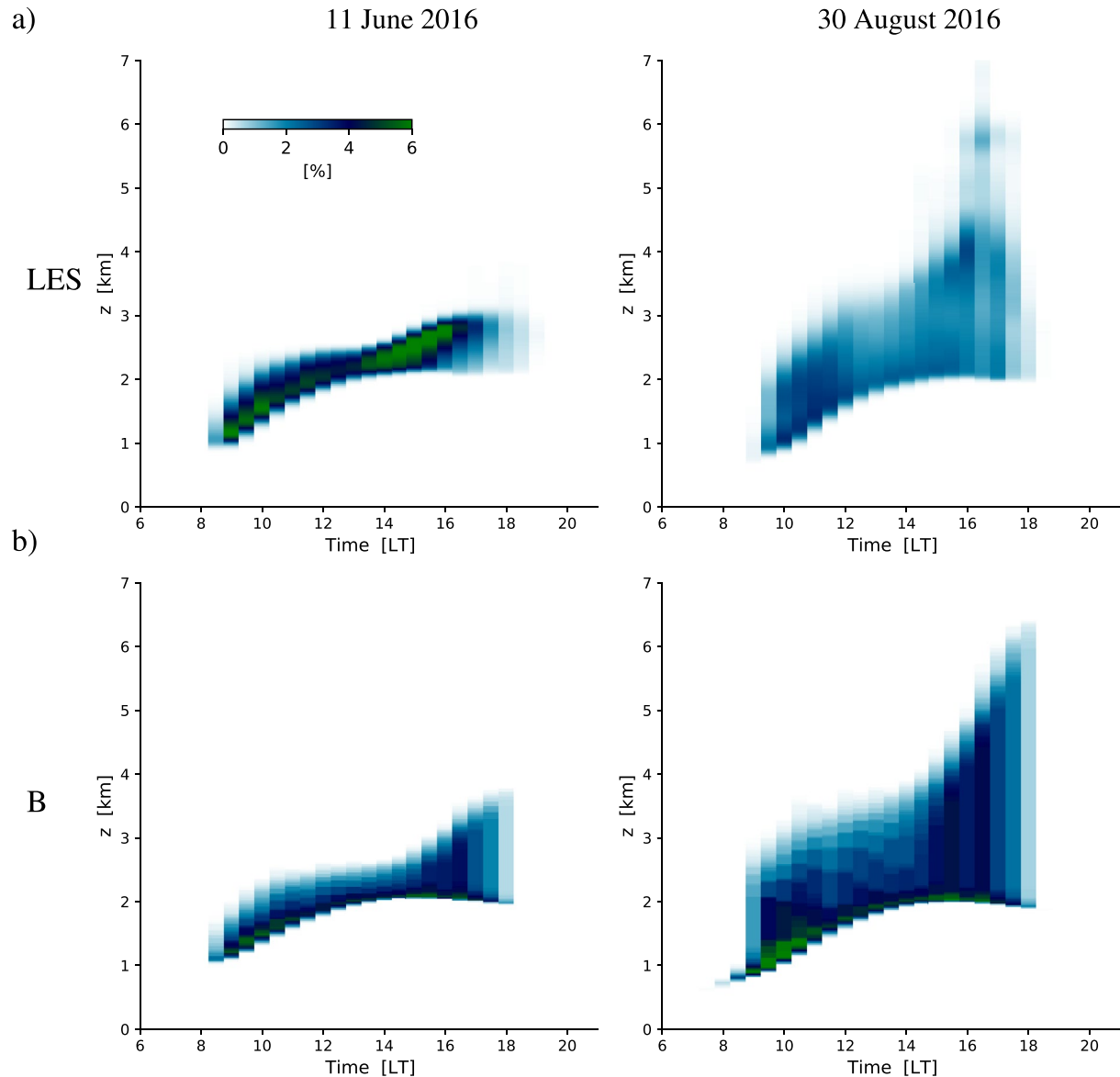
Figure 7. Time-height raster plots of cloudy area fraction in (a) LES and (b) BiOMi-ED(MF) n control experiment B. The left column shows results for 11 June 2016, the right column for 30 August 2016. For LES, the cloud core fraction is shown (defined as all cloudy point that are rising and have positive buoyancy), for EDMF, the condensed plume fraction. The data gridding represents 30 min averages.
