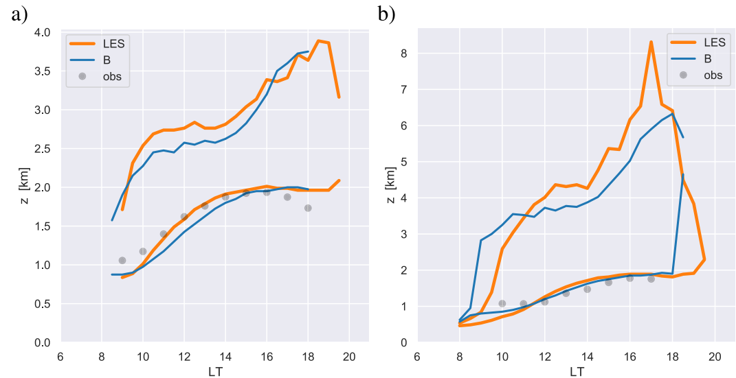
Figure 8. Time series of cloud base and top height (a) 11 June 2016 and (b) 30 August 2016. The control experiment B is shown in blue, the LES results in orange, and the gridded observations as part of the LASSO Data Bundle (v2) as gray dots.
