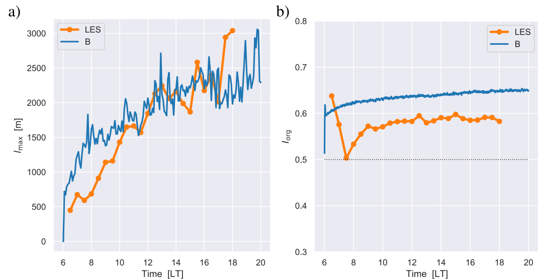
Figure 12. Time series of spatial statistics of the cluster population for 11 June 2016. (a) The largest cluster size l_{\text{max}} . (b) Organization metric I_{\text{org}} . Binomials On Microgrids (BiOMi) data for experiment B is shown in dark blue, and LES data in orange.
