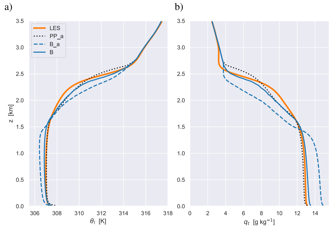
Figure 14. Same as Figure 9a but now showing \bar{\theta}_i and \bar{q}_i at 16:00 local time on 11 June 2016 for experiments PP_a (dotted black), B_a (dashed blue) and B (solid blue).
