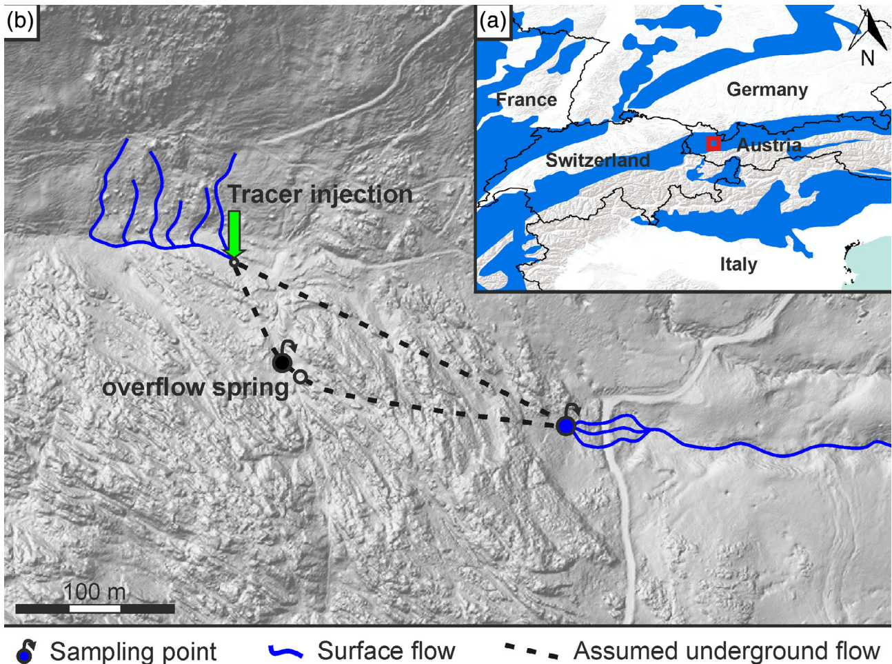
Figure 1. (a) Location of the test site in Western Austria (basemap: World Karst Aquifer Map; modified from Chen et al. [2017]); (b) detailed view of the karst experimental site (data from basemap: data.vorarlberg.gv.at).
