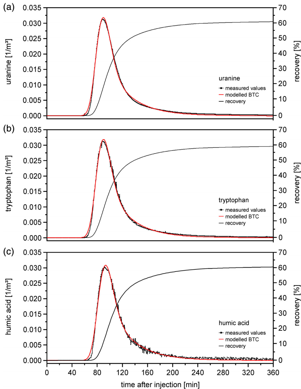
Figure 5. BTCs during low-flow conditions of (a) uranine, (b) tryptophan, (c) humic acid, each time together with the recovery and the modeled BTC.
