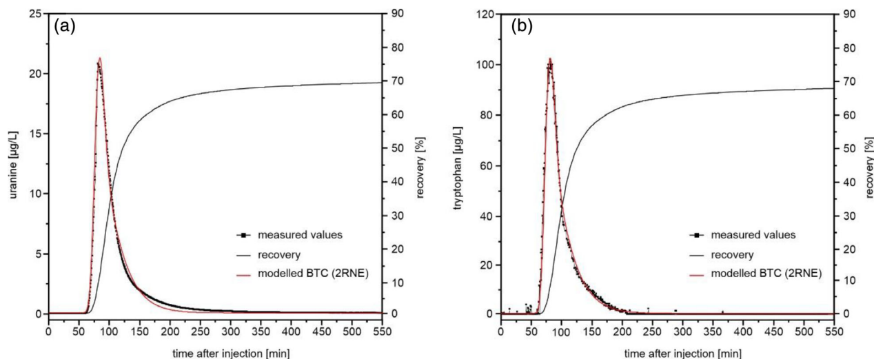
Figure A2. (a) BTC and recovery for uranine, discharge 14.5 L/s and (b) BTC and recovery of tryptophan, discharge 14 L/s.
