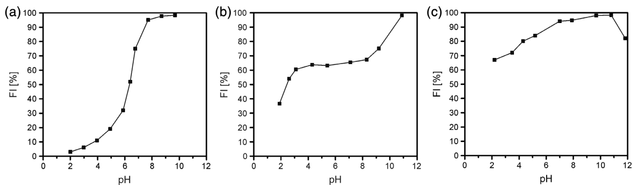
Figure 2. Dependency of the fluorescence intensity of the pH value for (a) uranine, (b) tryptophan, (c) humic acid; the highest measured fluorescence intensity was assumed as 100%.
