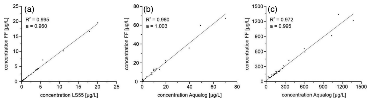
Figure A1. (a) Measured uranine concentration with the FF, compared to the measured concentration with the LS55 in the laboratory, (b) comparison of the measured tryptophan concentration of the FF and the Aqualog, and (c) comparison of the measured humic acid concentration with the FF and the Aqualog.
