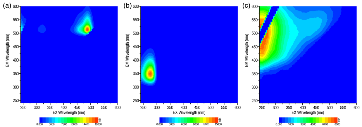
Figure 3. (a) EEM spectra of uranine recorded with the Aqualog, which shows \lambda_{ex} and \lambda_{em} of the main and secondary uranine fluorescence peak; (b) EEM spectra of tryptophan, which shows the main tryptophan fluorescence peak; (c) EEM spectra of humic acid.
