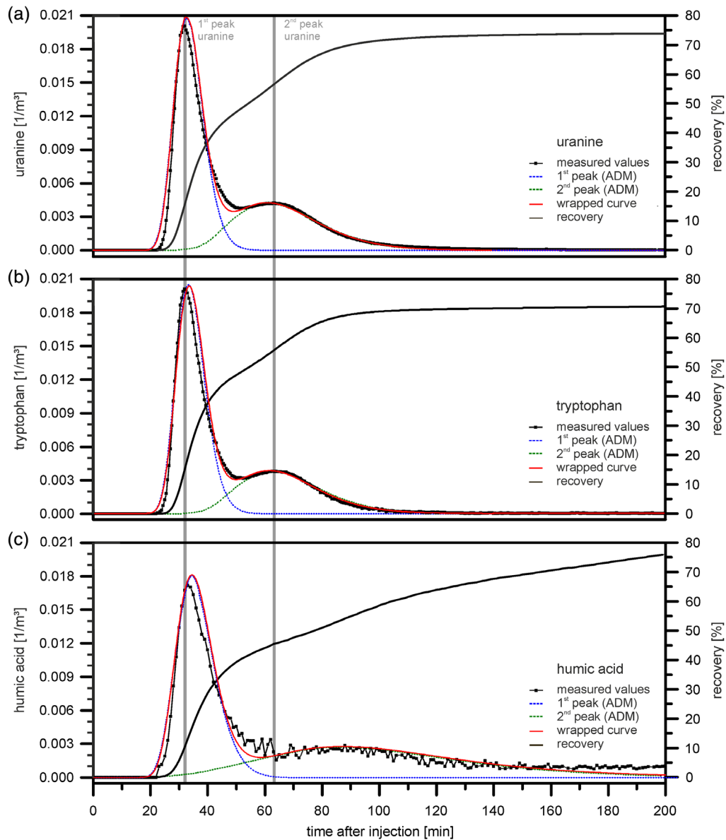
Figure 4. BTCs during mean- to high-flow conditions of (a) uranine, (b) tryptophan, (c) humic acid, each time together with the recovery and the modeled BTC for both peaks and the wrapped curve. Concentrations are normalized (c/M).
